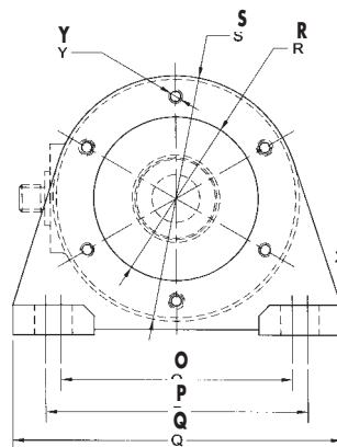
Mounting Bracket (with Slim Cell)
