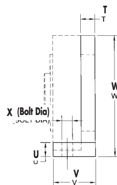
Mounting Bracket (with Slim Cell)
